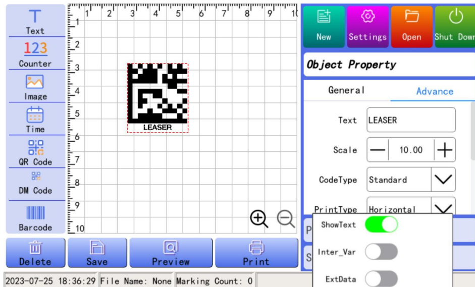
Figure 3.2.7.1 DM code editing
